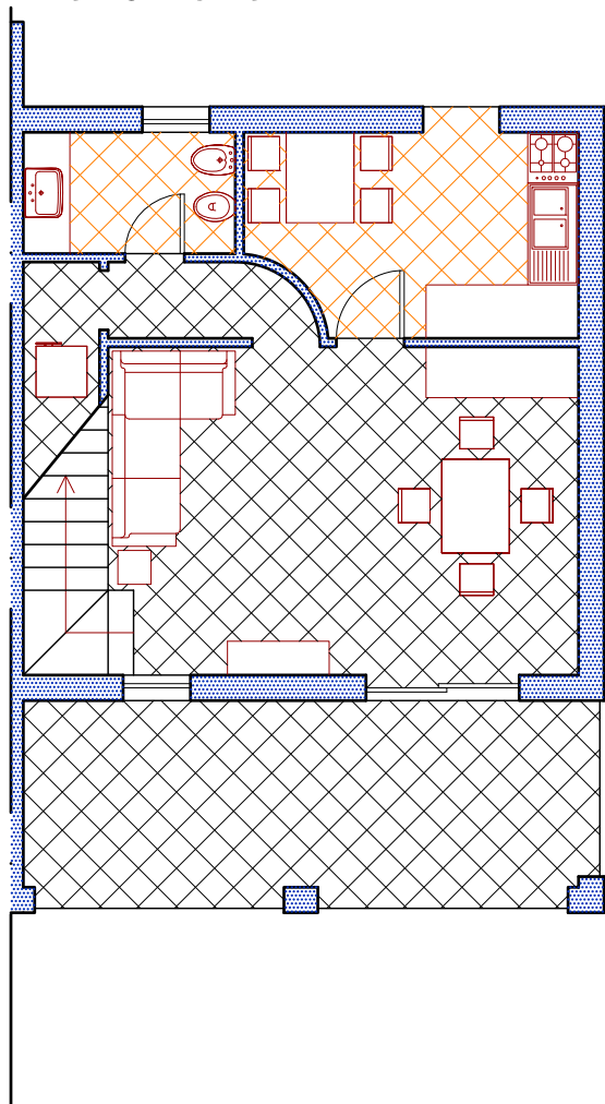
Piano Terra
